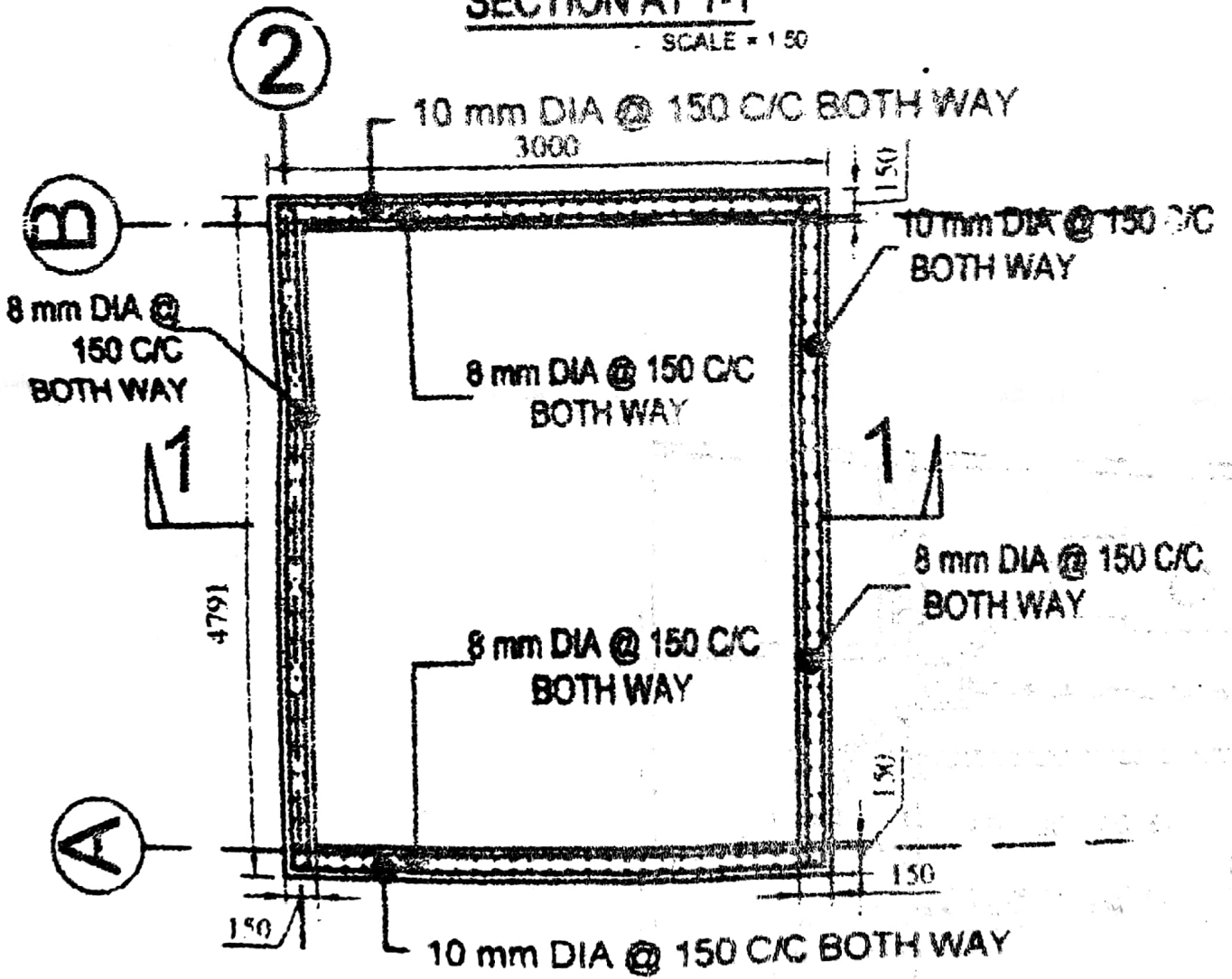
REINFORCEMENT DETAIL AND PLAN OF OVERHEAD RESERVOIR
