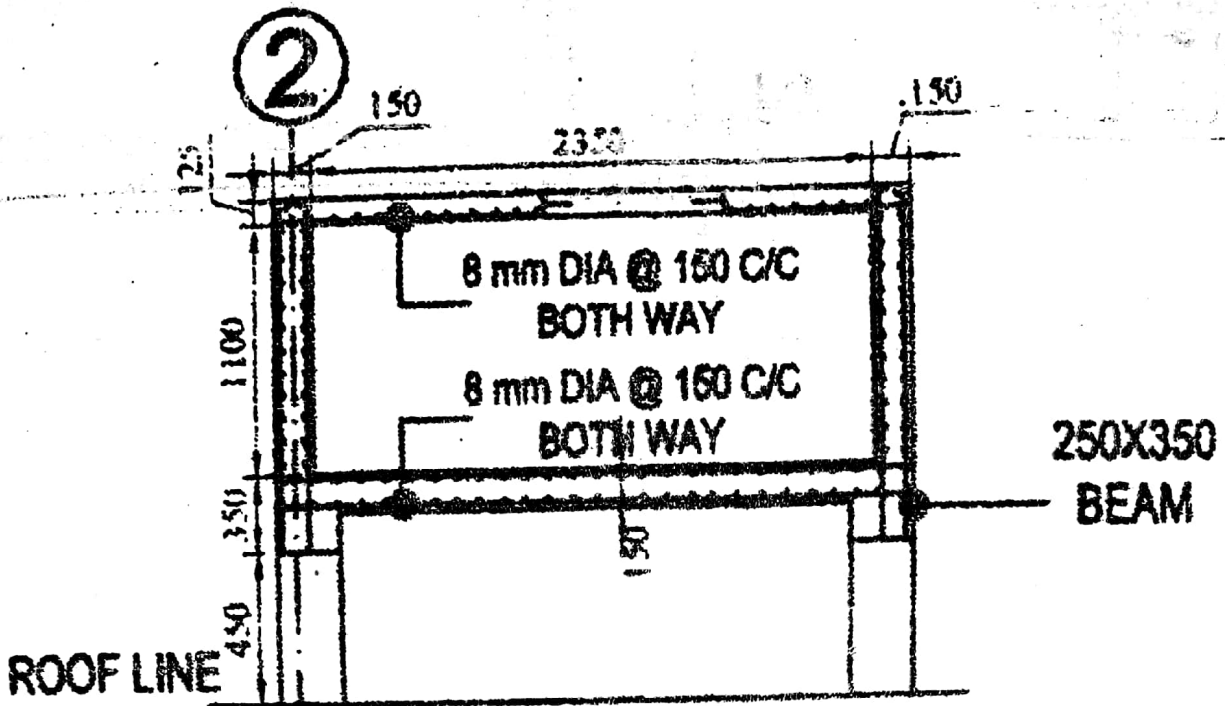
SECTION AT 1-1
